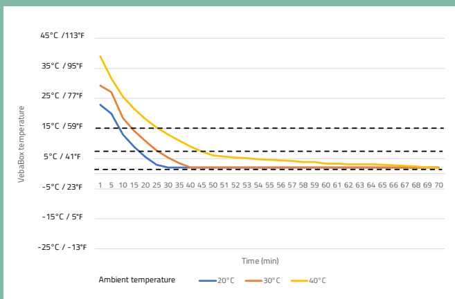
Cooling performance at different ambient temperatures >20°C / 68°F Model D Cool
