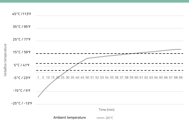
Heating performance at ambient temperature -20°C / -4°F Model D Cool
