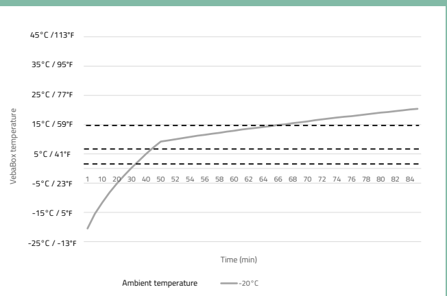
Heating performance at ambient temperature -20°C / -4°F Model F Cool
