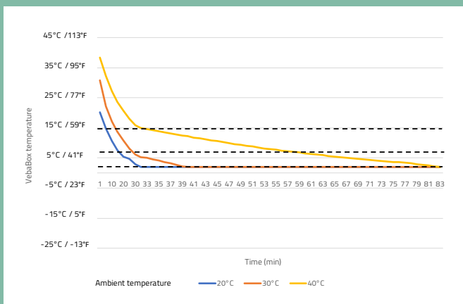
Cooling performance at different ambient temperatures >20°C / 68°F Model F Cool
