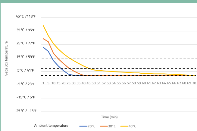
Cooling performance at different ambient temperatures >20°C / 68°F Model I Cool
