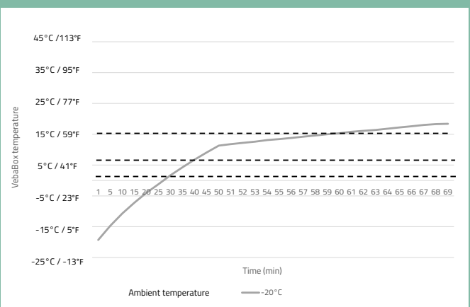
Heating performance at ambient temperature -20°C / -4°F Model I Cool
