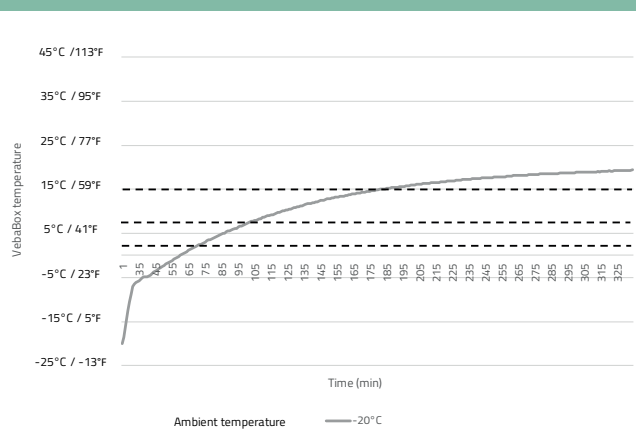
Heating performance at ambient temperature <0°C / 32°F Model S
