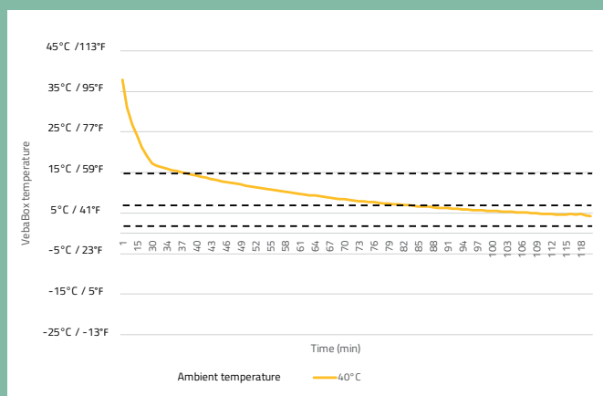
Cooling performance at ambient temperature >20°C / 68°F Model S
